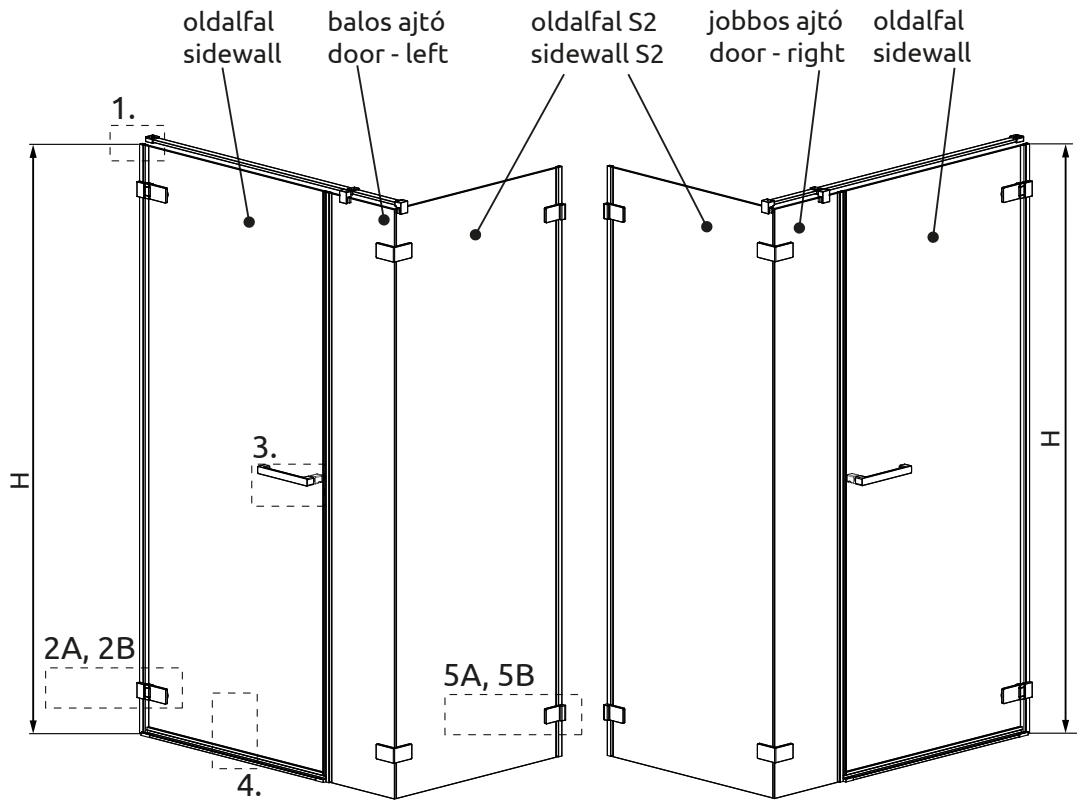
Balos kabin Variant L
